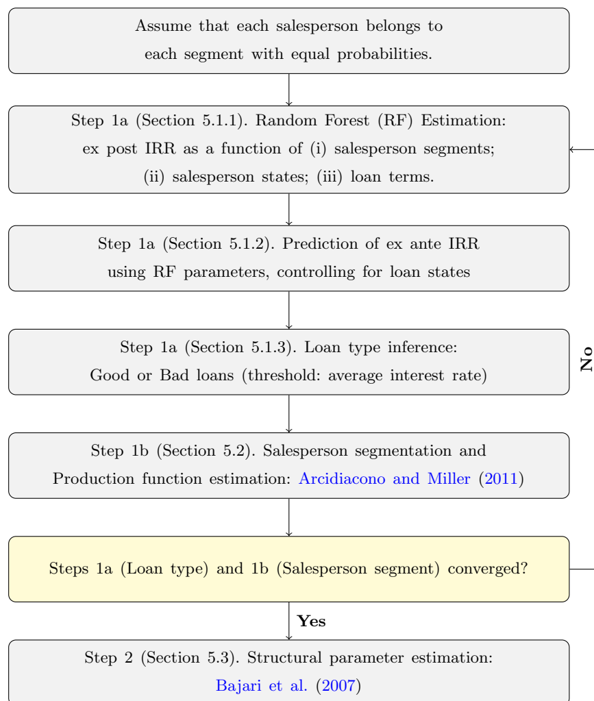
Figure 5 Estimation Overview
